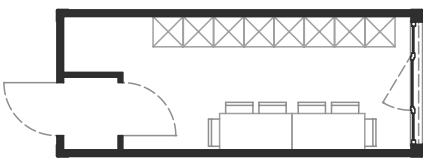
Modell 1U612 2802x2438x6058
