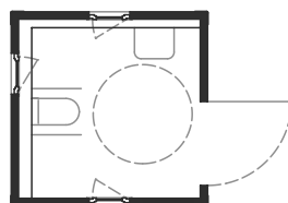
Barrierefreies-WC Modell 1H322 2802x2990x2990
