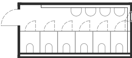
Damen-WC Modell 1W6222 2802x2990x6058
