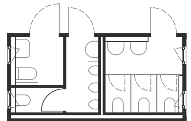
D.-/H.-/Barrierefreies-WC Modell 1H6223 2802x2990x6058
