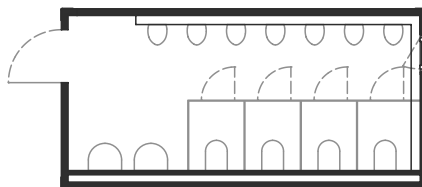
Herren-WC Modell 1W6221 2802x2990x6058
